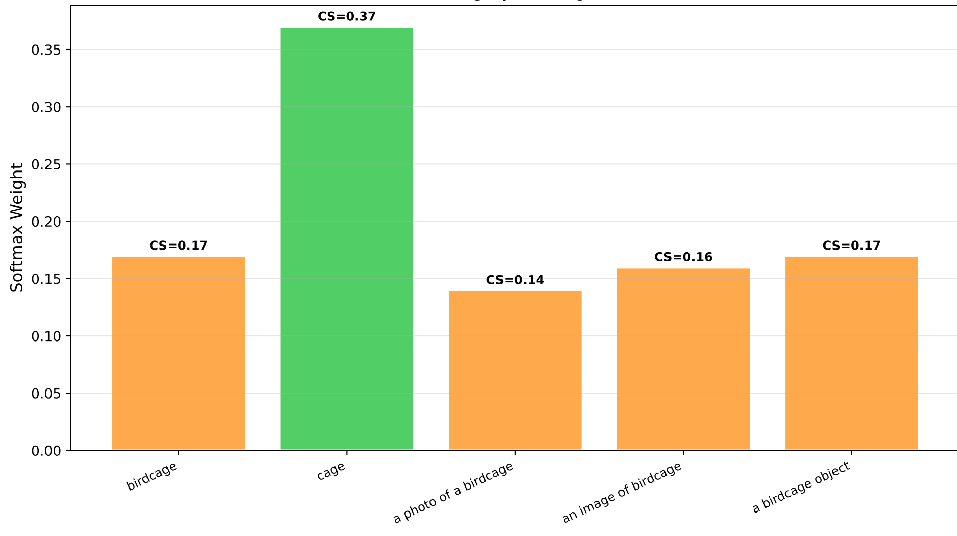
Softmax Weights by Complementarity Score Category: birdcage
